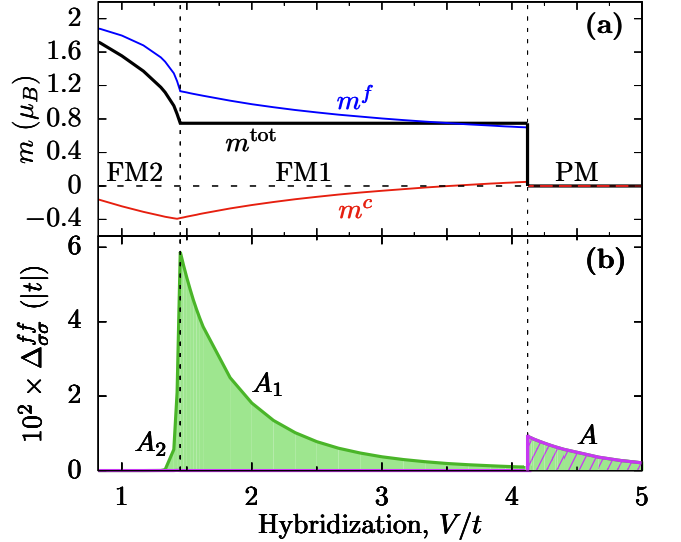
FIG. 3. Phase diagram for U/|t| = 4 , J/|t| = 1.6 , t'/|t| = 0.25 , temperature T/|t| = 10^{-8} and n^{\text{tot}} = 3.25 . (a) Total magnetic moment (black line) and f - and c -electron magnetizations (blue and red lines, respectively). (b) Superconducting gap parameters \Delta_{\downarrow\downarrow}^{ff} (green shading) and \Delta_{\uparrow\uparrow}^{ff} (purple shading).
