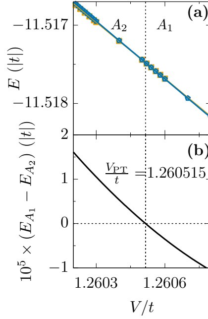
Figure D.10.: Energy difference between FM1+ A_1 and FM2+ A_2 phases for reduced magnetic field h/|t| = 0.002 .
