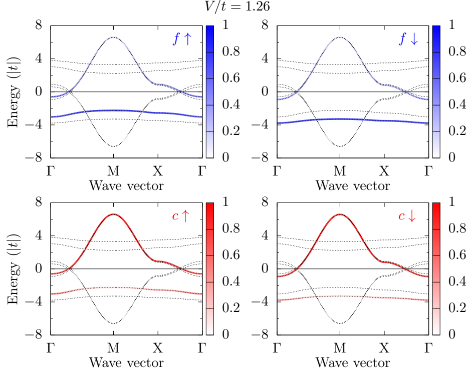
Figure D.2.: Band structure for V/t = 1.26 in the FM1+ A_1 phase. Colors the same as in Figure D.1.
