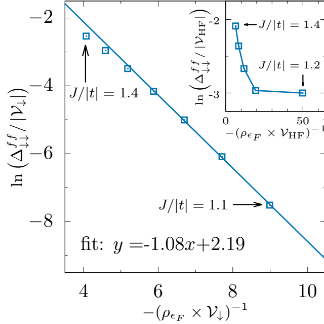
Figure 3.7.: BCS-type scaling for U/|t| = 3.5 and different Hund's coupling values J , for fixed hybridization V/t = 1.32 . Inset: failure of scaling with the Hartree-Fock-BCS pairing potential \mathcal{V}_{\text{HF}} = U' - J .
