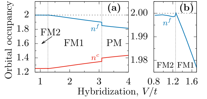
FIG. 4. (a) Occupancies of the f - and c -orbitals as a function of hybridization. (b) Close-up of the FM2→FM1 transition.
