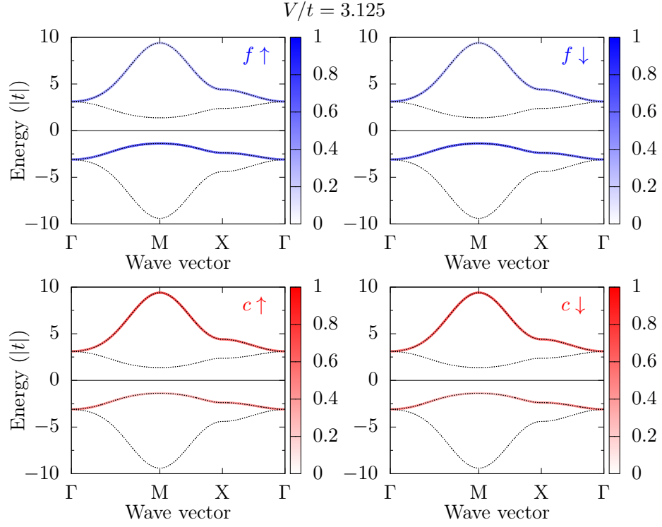
Figure D.3.: Band structure for V/t = 3.125 in the PM+ A phase. Colors the same as in Figure D.1.
