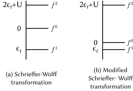
Figure 4.7.: Comparison of energy levels, which indicates the choice of the transformation type. In the left panel (a) both processes c + f^1 \leftrightarrow f^2 and f^1 \leftrightarrow f^0 + c involve high-energy scales; therefore, both of them are transformed out (the case of the Schrieffer-Wolff transformation ). In the right panel (b) the f -level is shallowly located. Thus, V/\epsilon^f cannot be treated as small perturbation. Such a situation requires here a division of hybridization term to low- and high-energy processes (as presented in Figure 4.2).
