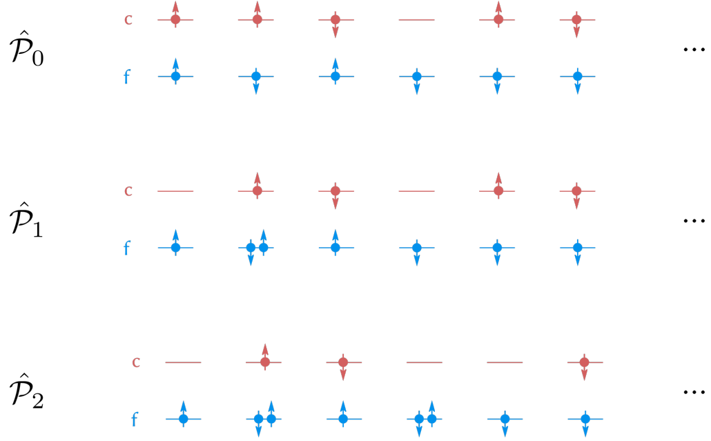
Figure 4.3.: Schematic description different local contribution to the projection operators (4.13) – (4.15). The operator \hat{\mathcal{P}}_0 suppresses double f -occupancies, whereas \hat{\mathcal{P}}_1 creates one additional double f -occupancy, and \hat{\mathcal{P}}_2 (4.15) creates two additional double f -occupancies in the system.
