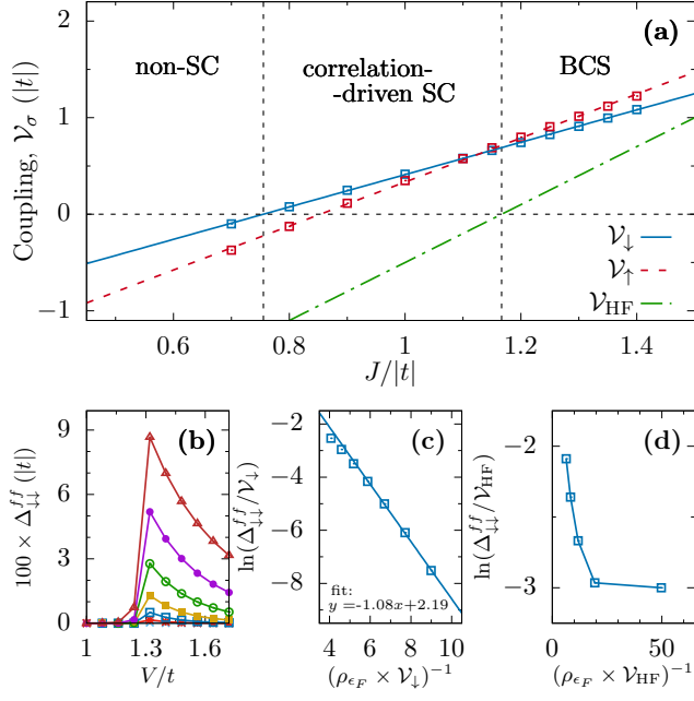
FIG. 3. (a) Dependence of V_\sigma on the Hund's coupling J for V/t = 1.32 (solid blue and dashed red lines). For comparison, the value of the Hartree-Fock (HF/BCS) coupling constant V_{\text{HF}} is also shown by green dash-dotted line. Black dashed vertical lines split the plot into three regions: non-SC, correlation-driven (where SC is not supported at the HF/BCS level, yet it appears due to correlation effects), and BCS regime (where SC phase emerges in the HF/BCS approximation). Note that the value J/|t| = 1.1 , considered above, falls into the correlation-driven regime. (b) Hybridization-dependence of the SC gap component \Delta_{\downarrow\downarrow}^{ff} for various J near the FM2→FM1 transition. Values of J/|t| (from top to bottom) are 1.4, 1.35, 1.3, 1.25, 1.2, 1.15, and 1.1. (c) Scaling of \Delta_{\downarrow\downarrow}^{ff} with the dimensionless effective coupling \rho_{e_F} V_\downarrow . Here \rho_{e_F} denotes total density of states per f -orbital per spin, evaluated at the Fermi energy in the normal phase. The gap follows renormalized BCS scaling \Delta_{\downarrow\downarrow}^{ff} \propto V_\downarrow \times \exp(-(\rho_{e_F} V_\downarrow)^{-1}) . (d) The same as in (c), but with HF/BCS coupling V_{\text{HF}} used instead of V_\downarrow . Breakdown of BCS scaling implies relevance of the correlation-driven coupling renormalization.
