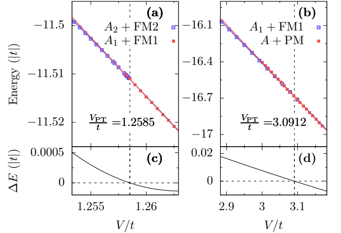
FIG. 1. Crossing of the energies near (a) FM2 + A_2 \rightarrow FM1 + A_1 and (b) FM1 + A_1 \rightarrow PM + A transition for U/|t| = 3.5 . Panels (c)-(d) show the energy differences \Delta E between extrapolated energies on both sides of respective phase transitions. The latter become zero at the transition point, denoted as V_{\text{PT}} , and are displayed in the plot. Model parameters coincide with those used in Fig. 1. of the main text.
