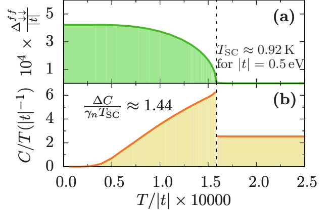
FIG. 2. Temperature-dependence of (a) gap parameter \Delta_{\downarrow\downarrow}^{ff} and (b) electronic specific heat for U/|t| = 3.5 , J/|t| = 1.1 , V/t = 1.3 , \epsilon^f/|t| = -4 , t'/|t| = 0.25 , and n^{\text{tot}} = 3.25 .
