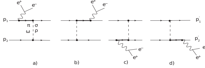
Figure 1.3: Bremsstrahlung diagrams for the process N_1 + N_2 \rightarrow N'_1 + N'_2 e^+ e^- , where N_1 and N'_1 stand for protons and N_2 and N'_2 denote nucleons, in the one photon and one-boson exchange approximation (thick lines denotes propagators of either nucleons or baryon resonances) [17].
