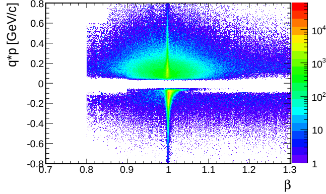
Figure 3.6: Experimental distribution of polarity \times momentum vs beta for e^+e^- with visible time of flight condition.
