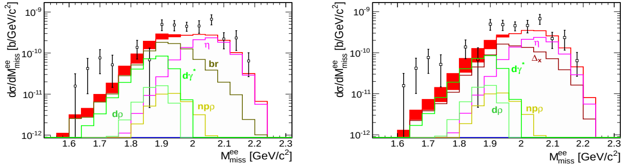
Figure 3.46: Missing mass of e^+e^- for M_{inv}^{e^+e^-} > 280\text{MeV} in the case when electron and positron and at least two protons are identified. Left picture contains bremsstrahlung, right one \Delta channel. Channels are described with colors in figures.
