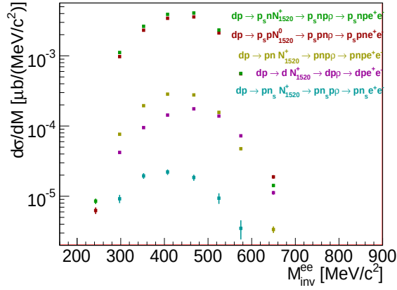
Figure 3.23: e^+e^- invariant mass distributions in HADES acceptance with the spectator condition and the e^+e^- opening angle \alpha_{e^+e^-} > 9^\circ for various reactions.
