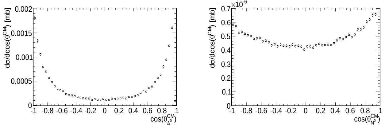
Figure 3.17: Angular \Theta distribution of resonans particle for d p \rightarrow p_{sp} n \Delta^+ (left) and d p \rightarrow p_{sp} p N^0(1520) (right).
