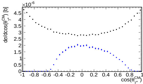
Figure 3.31: The simulated \cos(\theta_{\gamma^*}^{CM}) distribution for M_{inv}^{e^+e^-} < 140\text{MeV} in full solid angle (black) and inside HADES acceptance (blue).
