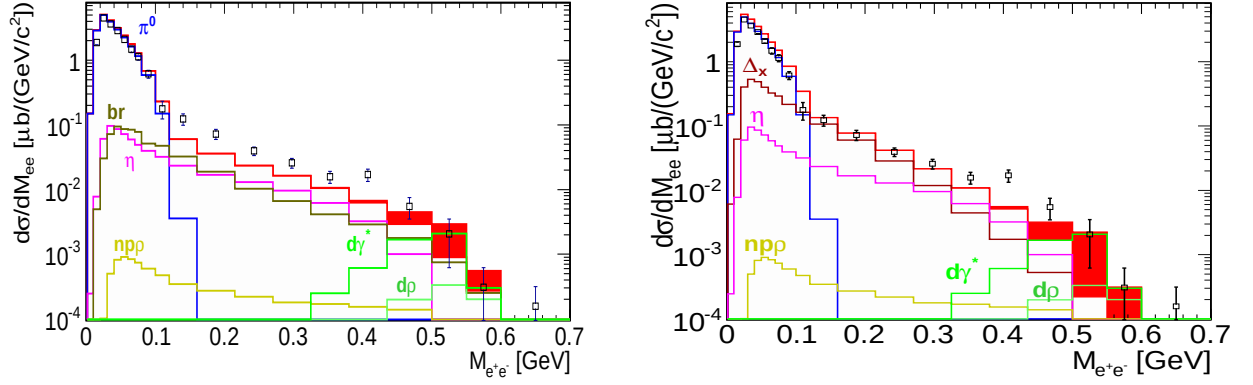
Figure 3.44: Invariant mass distribution of e^+e^- obtained for events with two hits in FW. Left: model "B". Right: model "A".
