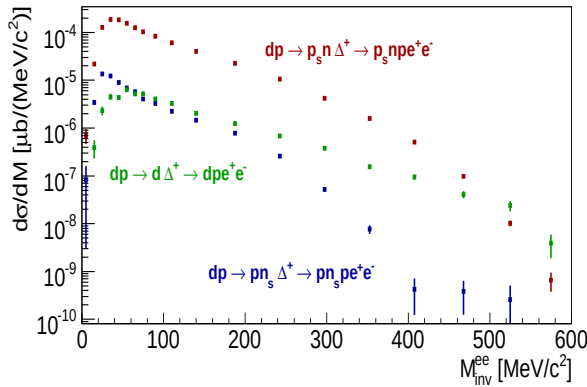
Figure 3.21: Invariant mass distribution of e^+e^- in HADES acceptance with spectator conditions and \alpha_{e^+e^-} > 9^\circ (see text). Types of channels are shown in the picture.
