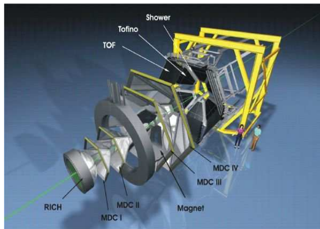
Figure 2.1: 3-dim view of the HADES detector.
