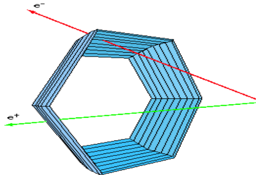
Figure 2.7: The Time Of Flight detector.
