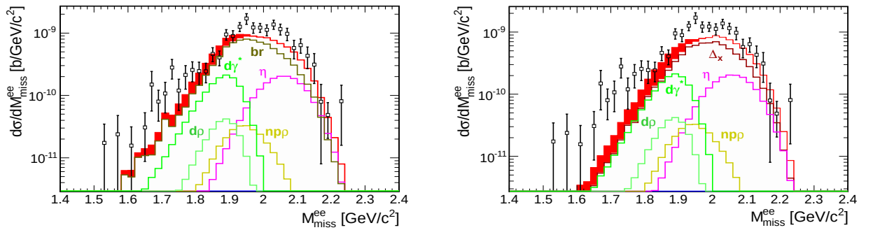
Figure 3.45: Missing mass of e^+e^- for M_{\text{inv}}^{e^+e^-} > 280\text{MeV} in the case when electron and positron and at least one proton are identified. Left picture contains bremsstrahlung, right one \Delta channel. Channels are described with colors in figures.
