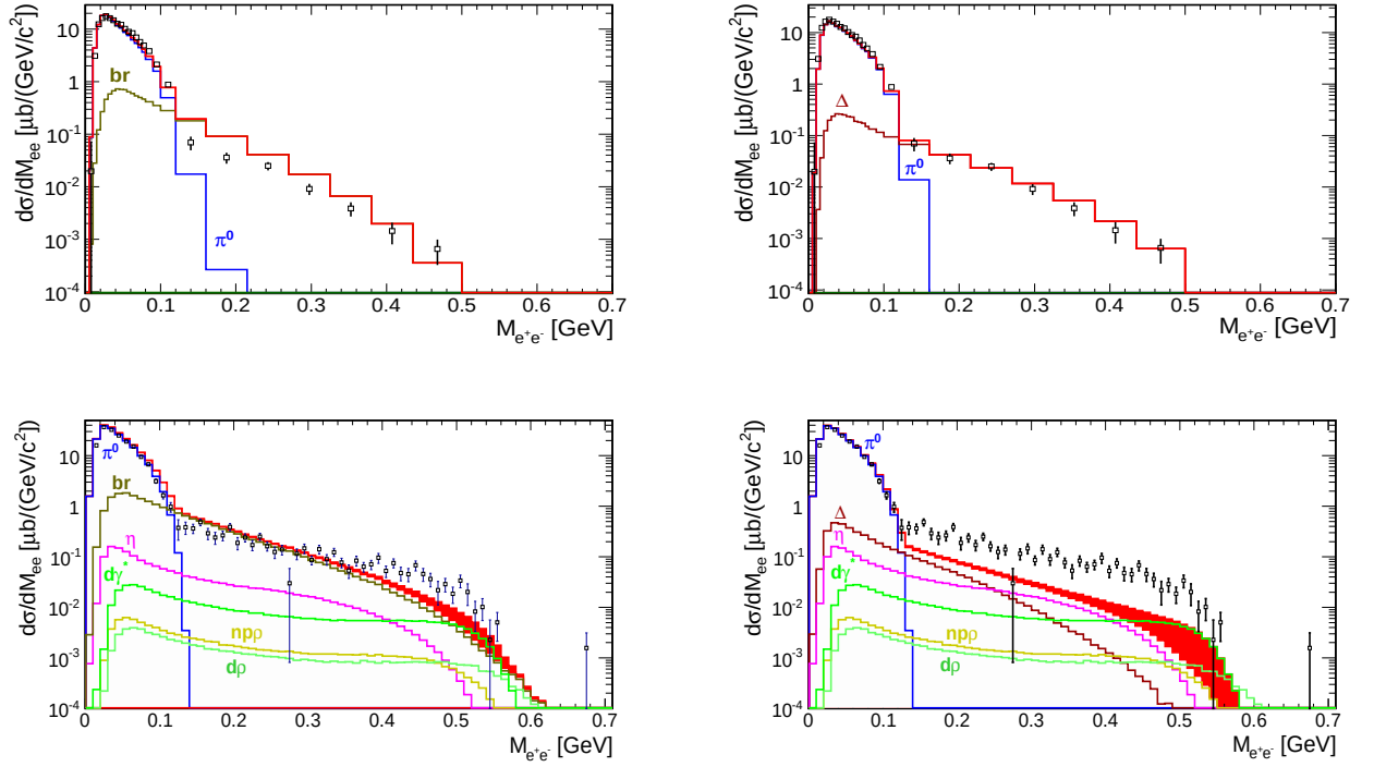
Figure 3.28: Invariant mass distribution of e^+e^- for p+p (up) and d+p (down) reaction at 1.25A\text{GeV} . Black squares represent experimental data and red line - sum of the contributions: \pi^0 (blue), \Delta (dark red), bremsstrahlung (brown), \eta (pink), \rho channels (yellow and green). Left hand side distribution contains bremsstrahlung and right hand side \Delta channel.
