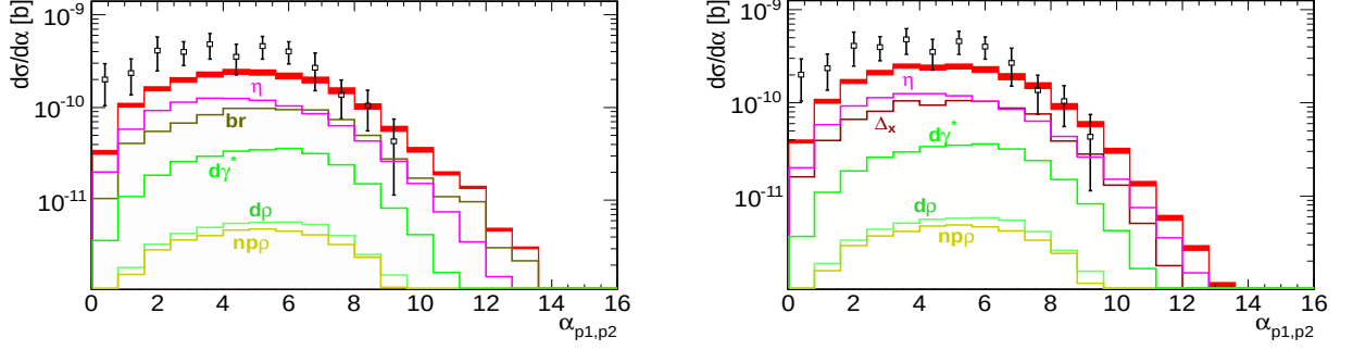
Figure 3.48: Opening angle between protons in FW for M_{inv}^{e^+e^-} > 280 \text{ MeV} .
