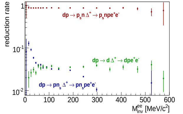
Figure 3.22: Reduction rate of survived dilepton pairs after additional spectator condition as a function of e^+e^- invariant mass for various reaction channels.
