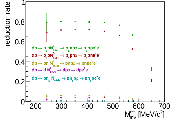
Figure 3.24: Rate of survived dielectron pairs after additional spectator condition as a function of the e^+e^- invariant mass for various reactions.
