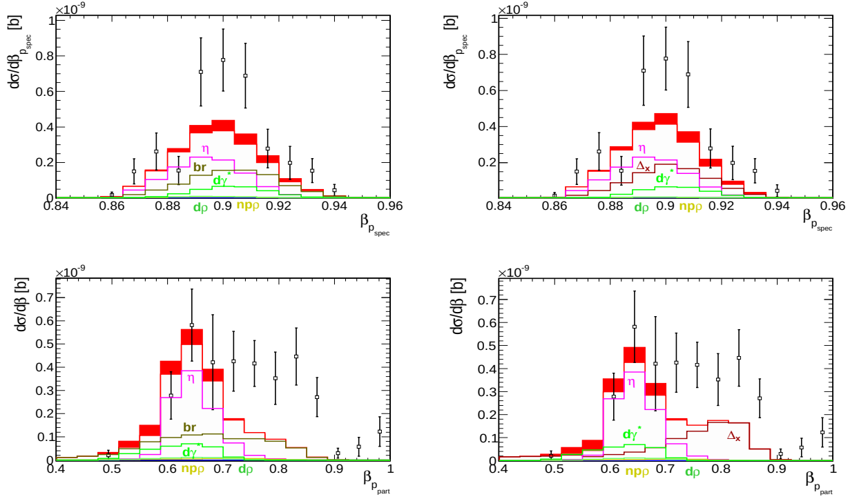
Figure 3.47: Velocity of proton spectator (upper figures) and proton participated in the reaction (lower figures) for M_{inv}^{e^+e^-} > 280 \text{ MeV} .
