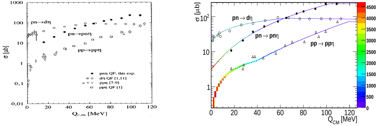
Figure 3.18: Left: total cross section for the \eta meson production as a function of the excess energy in c.m. system: p + n \rightarrow d\eta (open circles); p + n \rightarrow pn\eta (solid points); p + p \rightarrow pp\eta (open squares) [38]. Right: fits to the experimental data, where colors show abundance of events at the given energy.
