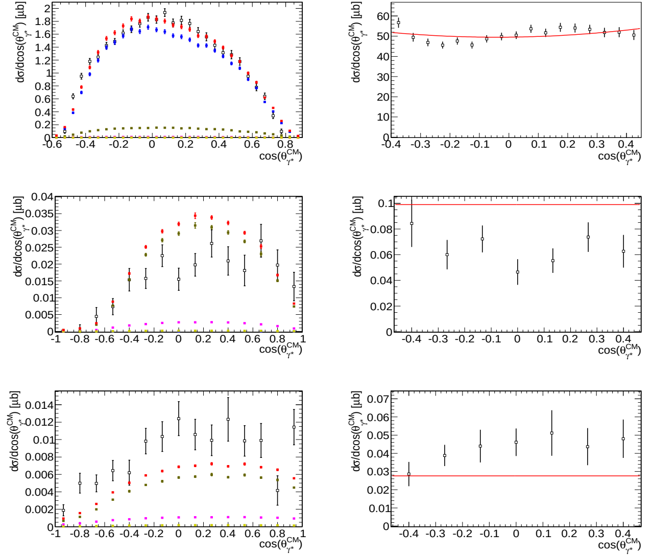
Figure 3.33: The comparison of \cos(\theta_{\gamma^*}^{CM}) for simulated (blue - \pi , brown - bremsstrahlung, pink - \eta , yellow - \rho , red - total) and experimental data (black points) in the HADES acceptance (l.h.s.) and acceptance corrected (r.h.s., where total simulation spectra is fitted with the red line) for different masses. First row: M_{inv}^{e^+e^-} < 150 \text{ MeV}/c^2 ; second: 150 \text{ MeV}/c^2 < M_{inv}^{e^+e^-} < 280 \text{ MeV}/c^2 ; last row: M_{inv}^{e^+e^-} > 280 \text{ MeV}/c^2 .
