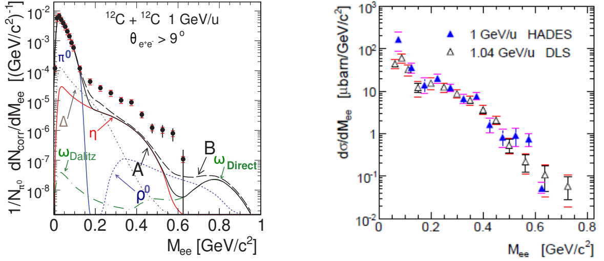
Figure 1.8: Left: e^+e^- invariant mass distribution in the reaction ^{12}C + ^{12}C at 1 A GeV by HADES after efficiency correction and normalization compared with model. Right: direct comparison of the dielectron cross sections measured in this reaction by HADES (full triangles) and at 1.04 A GeV by DLS (empty triangles) within the DLS acceptance [32].
