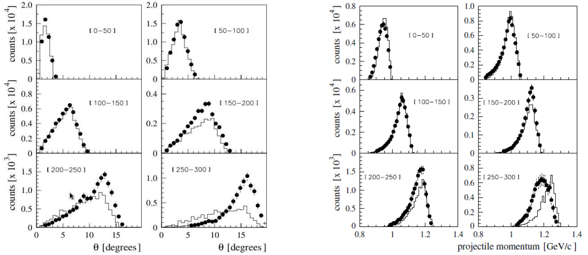
Figure 1.10: Experimentally deduced angular distribution of the spectator proton in the laboratory system (left) and effective neutron projectile momenta (right) for indicated relative momentum inside deuterium (given in \text{MeV}/c ) in comparison with Monte Carlo data [36]. Note changing y-axis scale.
