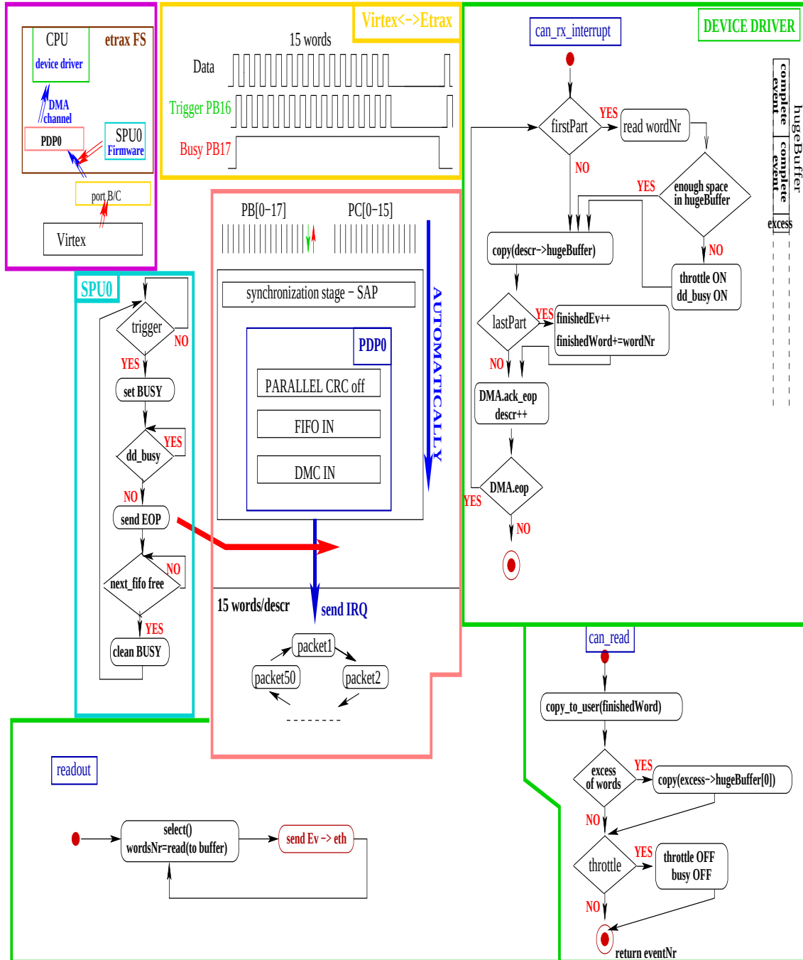
Figure A.6: The data flow diagram.
