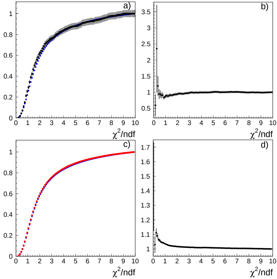
Figure 7.1: a) The cumulative curves of the \chi^2_{fit}/ndof distributions for the simulated K_S \rightarrow 3\pi^0 (black squares) and K_S \rightarrow 2\pi^0 (blue circles) samples and b) their ratio; c) Comparison of \chi^2_{fit}/ndof cumulative curves obtained with data (red squares) and simulations (blue circles) for the four gamma events and d) their ratio.
