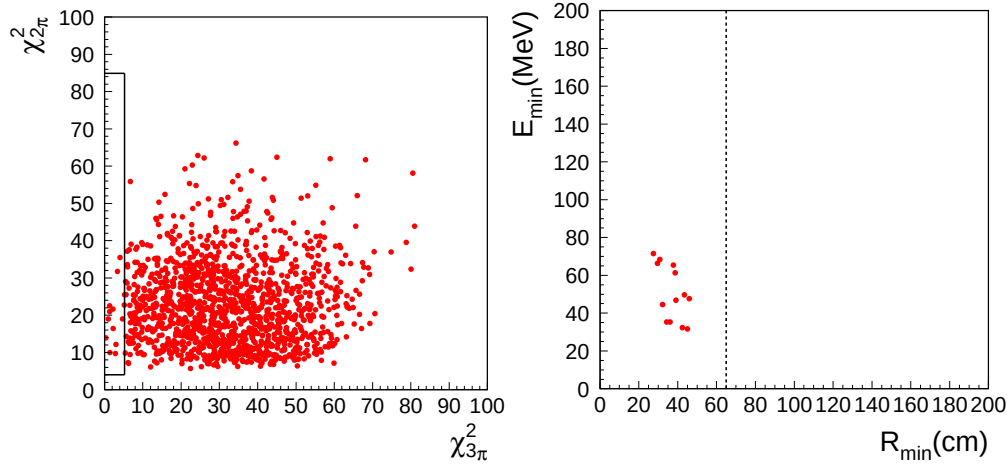
Figure 6.11: Experimental (\chi^2_{3\pi}, \chi^2_{2\pi}) distribution after the \chi^2 and \Delta E/\sigma_E cuts (left). The right panel presents the scatter plot of R_{min} versus the minimum energy of the cluster E_{min} for events in the Signal Box at the last stage of the analysis. The lines are described in the text.
