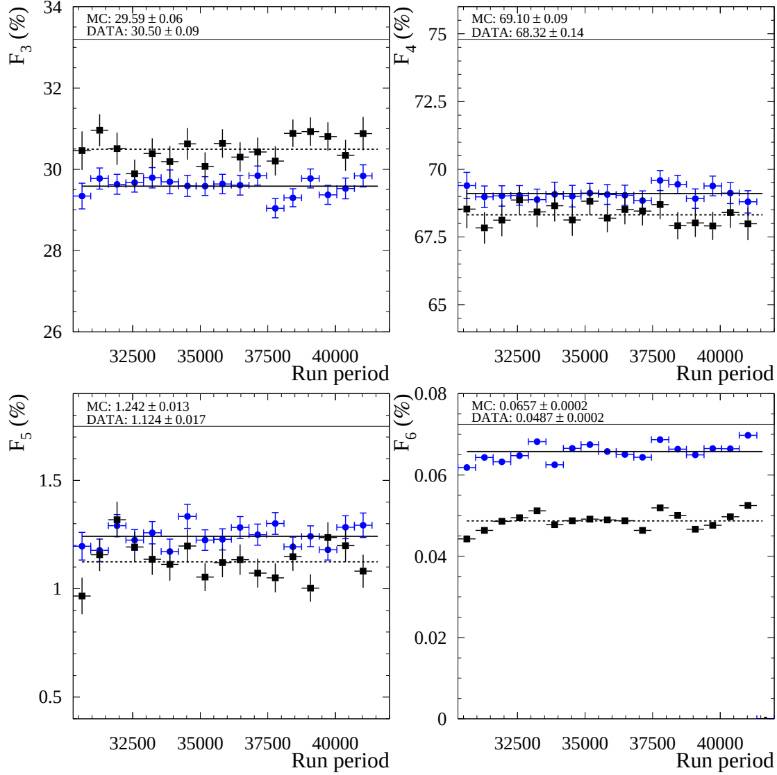
Figure 5.4: Comparison of the F_k distributions for data (black squares) and background simulations (blue circles). The solid and dashed lines denotes linear fits ( F_k = \text{const.} ) to the spectra of simulations and data, respectively. The results of the fit are reported on the top of each distribution.
