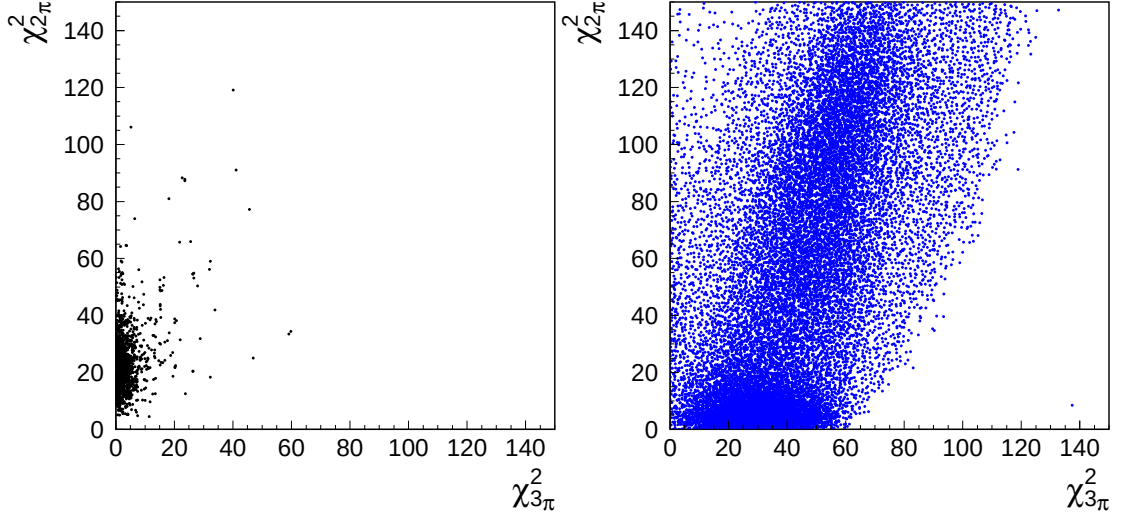
Figure 6.5: Scatter plot of \chi_{2\pi}^2 versus \chi_{3\pi}^2 for simulated K_S \rightarrow 3\pi^0 signal (left) and for the background after rejection of the \phi \rightarrow K_S K_L \rightarrow \pi^+ \pi^-, 3\pi^0 events (right).
