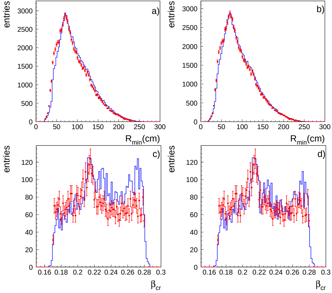
Figure 6.10: The inclusive distributions of R_{min} before (a ) and after (b ) correction. Plots c and d present \beta_{cr} spectrum for events with charged particles before and after the correction, respectively. The red points represent the data, while blue histograms denote simulation results.
