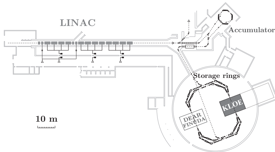
Figure 3.1: Schematic view of the DAΦNE collider. The picture was adopted from [20].
