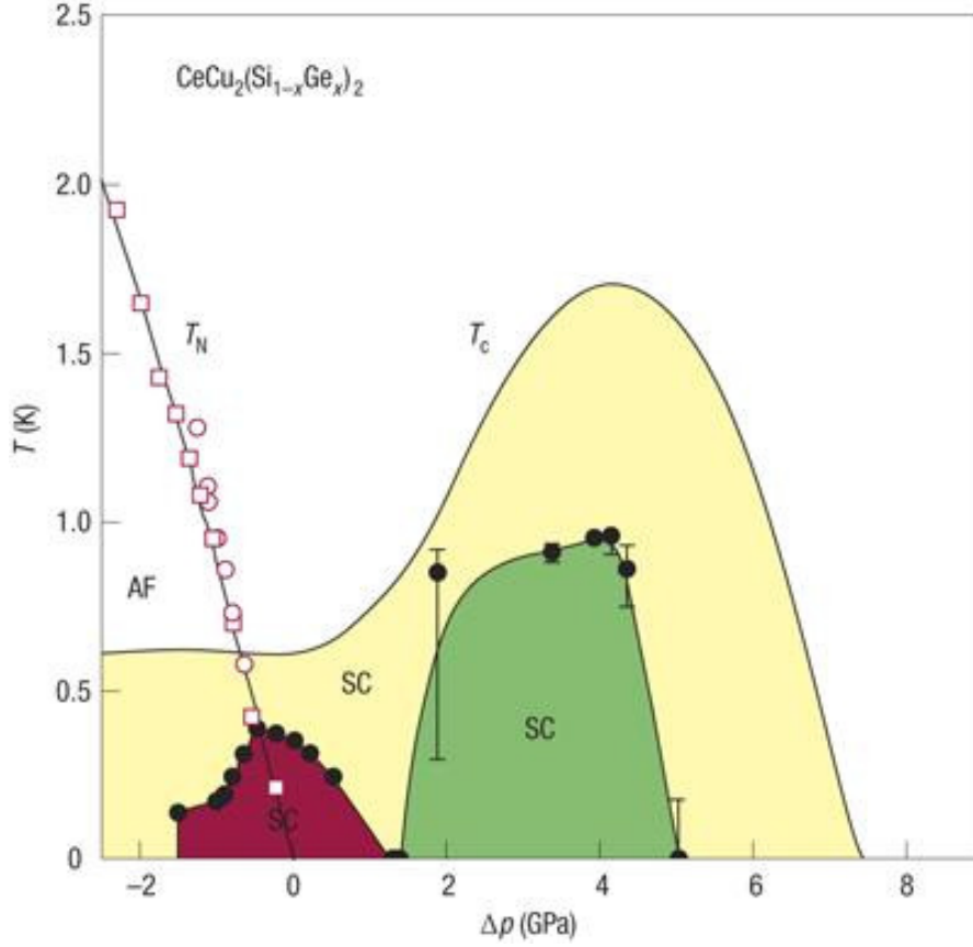
Figure 1.7: Phase diagram of the \text{CeCu}_2(\text{Si}_{1-x}\text{Ge}_x)_2 revealing two distinct superconducting domes (after Ref. [97]).
