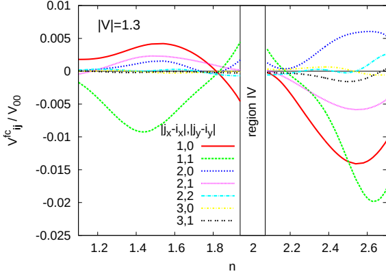
FIG. 8: (Color online) Spatial contributions V_{ij}^{cf} to the effective hybridization normalized by the first onsite ( i = j ) V_{00} term along the marked vertical line of the diagram in Fig.7a for |V| = 1.3 . Note that due to correlation initially local, on-site hybridization acquires effectively momentum dependence. However, the nonlocal contributions constitute only up to 2% of the local one.
