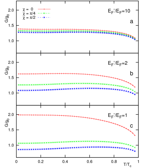
Fig. 2. Normalized ZBC as a function of the temperature for selected barrier strengths, \chi . The plots in parts (a), (b), (c) differ with the FLM. For specific values of barrier strength, we obtain flat maximum (parts (b), (c)).
