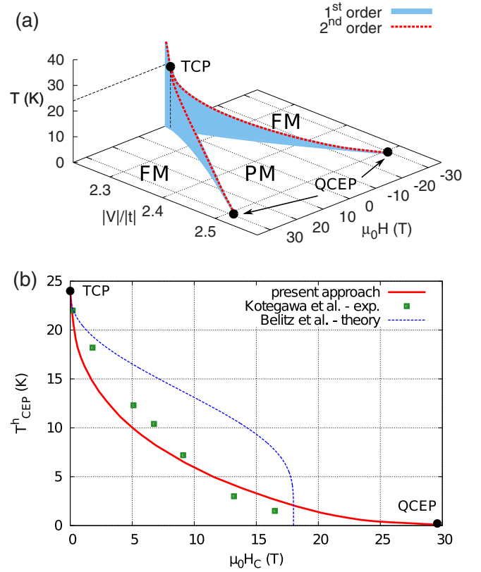
FIG. 3. (Color online) (a) Wing structure of the phase transition planes derived from our model. (b) Comparison of the calculated dependence of the temperature vs. applied magnetic field at the critical end point (CEP) with the experimental points adopted from [9]. For comparison, we include also the prediction by Belitz et al. [16], with the fitting parameters selected on the basis [9]: H_{QCEP} = 18 T and T_{TCP} = 24 K.
