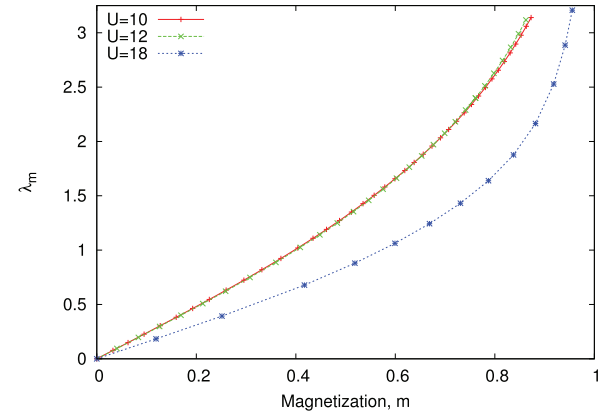
Figure 8. Effective field induced by correlations as a function of the magnetization; this illustrates its nonlinear character and in this manner it cannot be regarded as a Weiss molecular field.
