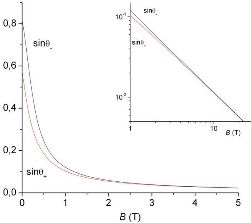
Fig. 1.7. Mixing parameters of electronic and nuclear angular momenta \sin\theta_+ and \sin\theta_- as a function of the magnetic field. At 1.5 T, \sin\theta_+ = 0.07128 and \sin\theta_- = 0.07697 .
