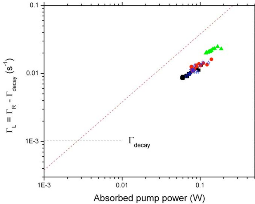
Fig. 3.27. Laser-induced relaxation rate \Gamma_L = \Gamma_R - \Gamma_{\text{decay}} , during OP experiments performed at 96 mbar (filled symbols) and different laser power (squares: 0.5 W, circles: 0.9 W and triangles: 2W) and 67 mbar with 500 mW (open stars). The horizontal dotted line represents the decay rate found for these experiments and the dashed line a guide for the eye fitting all the values obtained at low magnetic field.
