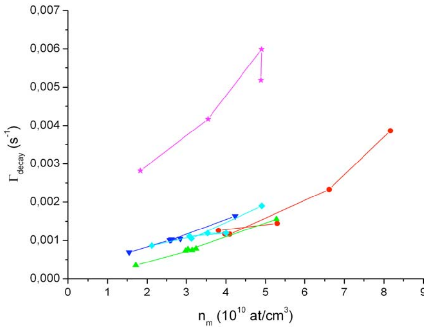
Fig. 3.21. Compiled decay rates \Gamma_{\text{decay}} = 1/T_{\text{decay}} in the discharge as a function of metastable densities measured at M = 0 with a weak pump beam before and after experiments. The results are sorted in function of the pressure: 32 mbar (circles), 67 mbar (triangles), 96 mbar (reversed triangles), 128 mbar (diamonds) and 267 mbar (stars).
