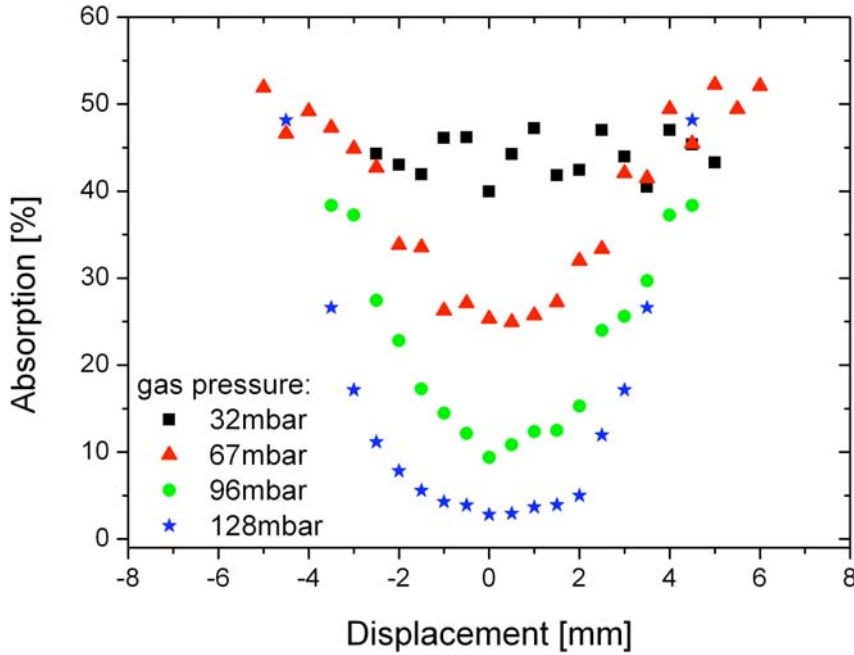
Fig. 3.5. Comparison between laser absorption profiles collected for various ^3\text{He} gas pressures. The measurements were done at 2 T.
