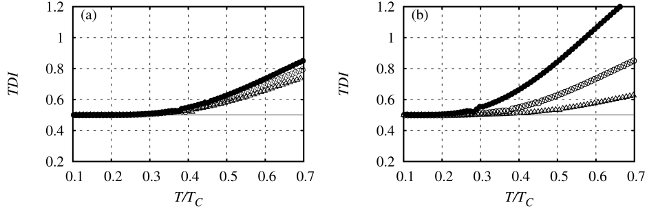
Figure 4.5: The evolution of TDI for different pair-interaction energies. (a) V_{AV} = 0.04 [eV]: E_{asym} = 0.06 [eV] - filled circles; E_{asym} = 0.07 [eV] - empty circles; E_{asym} = 0.06 [eV] - empty triangles; (b) E_{asym} = 0.07 [eV]: V_{AV} = 0.3 [eV] - filled circles, V_{AV} = 0.4 [eV] - empty circles, V_{AV} = 0.5 [eV] - empty triangles; Solid lines in both figures refer to 1/2 level.
