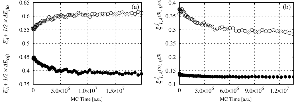
Figure 5.21: The energetic barriers (in [eV]) for an A-atom jumps (a) and \xi_{I:A}^{j(B)} - V^{(\alpha)} SRO parameters (b) for T/T_C = 0.53 : filled circles - formation of antisite jump ( A : \alpha \rightarrow \beta ); empty circles - reversal jumps ( A : \beta \rightarrow \alpha )
