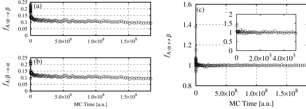
Figure 5.18: A-atom jump frequencies (a,b) and the ratio between them (c) in a function of MC time, collected for T/T_c = 0.37 .
