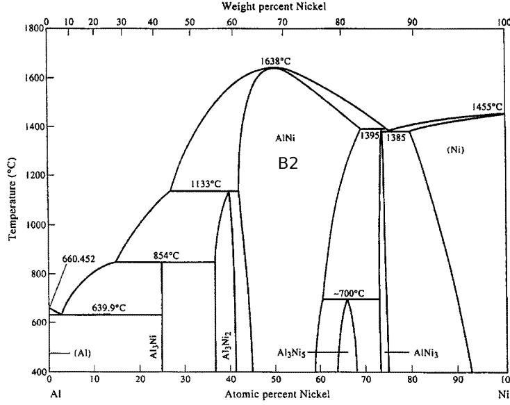
Figure 1.3: Ni - Al system phase diagram [7].
