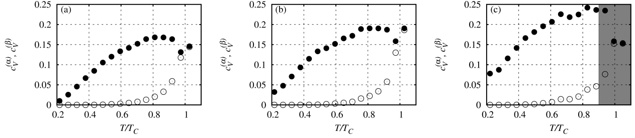
Figure 4.16: Temperature dependencies of vacancy concentrations on sub-lattices in a) A_{0.52}B_{0.48} ; (b) A_{0.5}B_{0.5} ; (c) A_{0.48}B_{0.52} ; “ \alpha ” sub-lattice - filled circles, “ \beta ” sub-lattice - empty circles.
