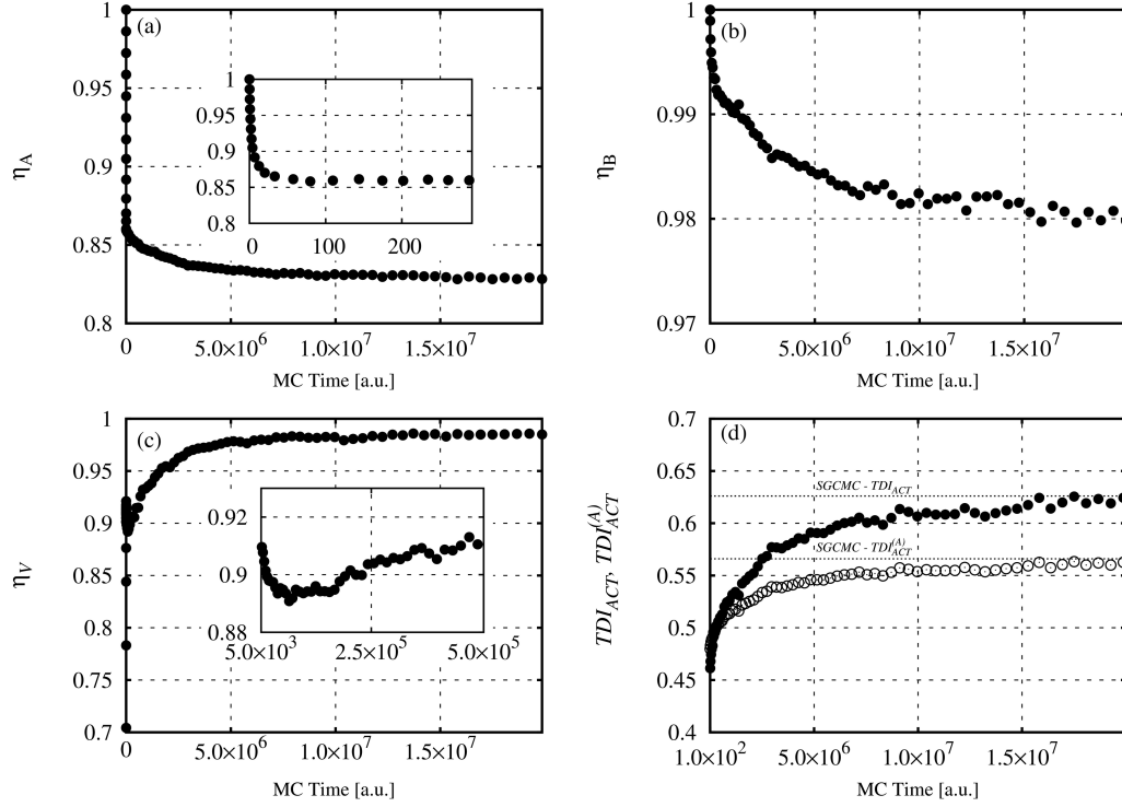
Figure 5.12: The LRO parameters (a,b,c) and triple defect indicators (d) at temperature T/T_C = 0.53 . Dotted lines indicate equilibrium values obtained in SGCMC (d).
